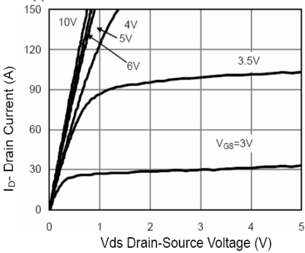
Output Characteristic
