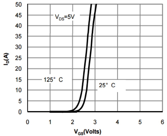
Transfer Characteristic
